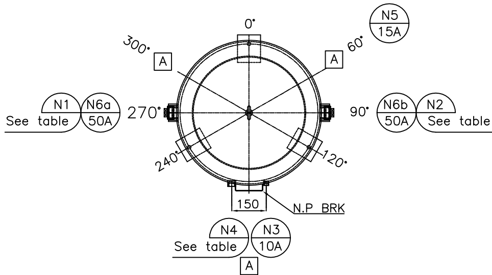
NOZZLE ORIENTATION
